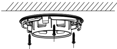
Figure 2-5 Secure the Mounting Base
