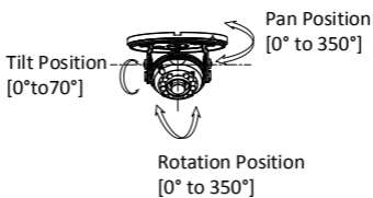
Figure 2-14 3-Axis Adjustment
